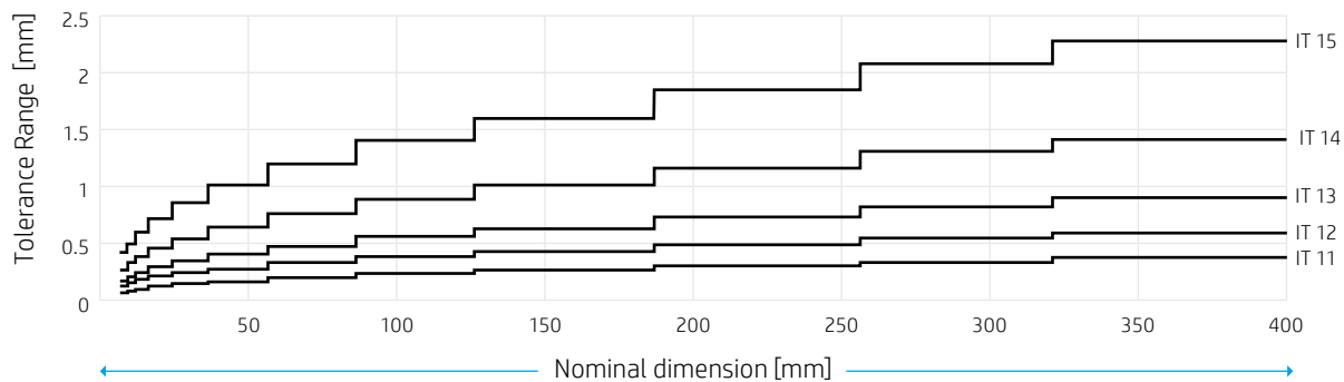
Figure 5. Tolerance range vs. dimension length
